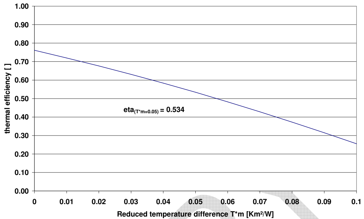
Fig A1.6: Efficiency curve for 1000 W/m 2 Global irradiation and a fraction of 15% diffuse irradiation
